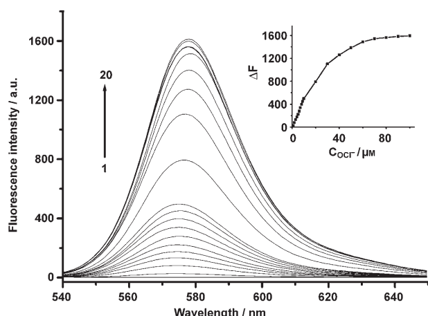
Figure 5. Fluorescent spectra of probe 1 (10 μM, curve 1) and its reaction solutions with various concentrations of \text{OCl}^- (1–100 μM, curves 2–20) according to the general procedure. The inset shows the plot of fluorescence enhancement value \Delta F against \text{OCl}^- concentration.
