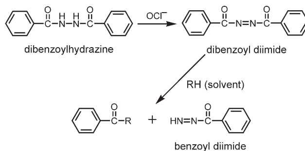
Scheme 1. The \text{OCl}^- anion oxidizes dibenzoylhydrazine into dibenzoyl diimide.
