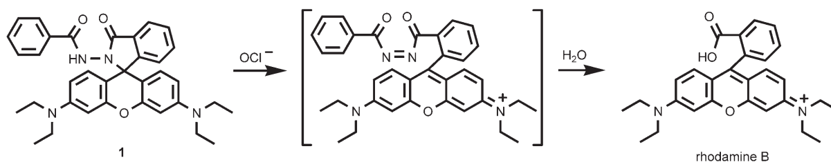
Scheme 4. The possible ring-opening reaction of 1 that is induced by the oxidative action of \text{OCl}^- .
