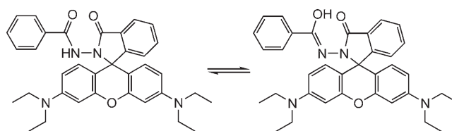
Scheme 3. Two possible tautomers of probe 1 .
