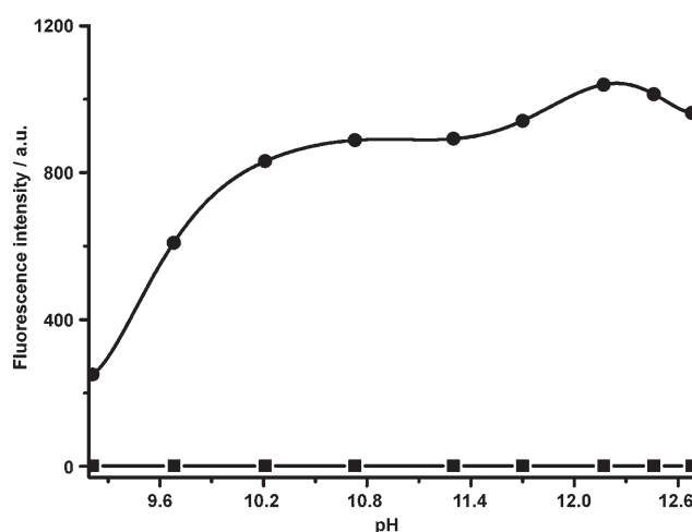
Figure 4. Effect of pH on the reaction of 1 ( 10\text{ }\mu\text{M} ) with \text{OCl}^- ( 40\text{ }\mu\text{M} ); 1 + \text{OCl}^- (●), 1 (■). Fluorescence intensity was measured at \lambda_{\text{ex/em}}=520/578\text{ nm} .
