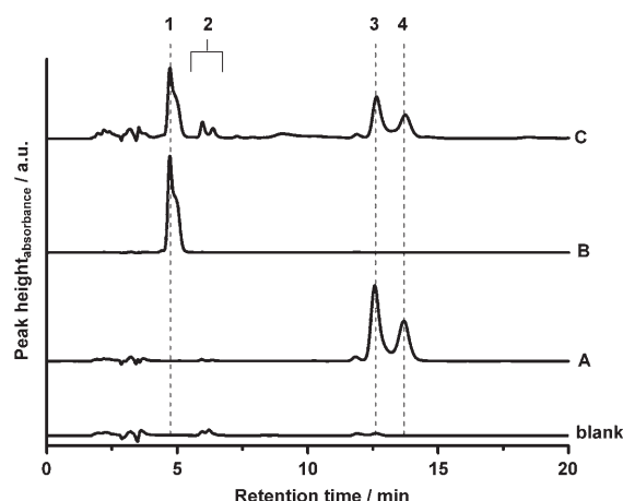
Figure 6. HPLC chromatograms of different reaction products in 0.03 M \text{Na}_2\text{B}_4\text{O}_7/\text{NaOH} buffer (pH 12) that contained 30% THF. A) 100 μM probe 1 , B) 100 μM rhodamine B, C) 100 μM 1 plus 100 μM \text{OCl}^- , and (blank) 100 μM \text{OCl}^- . HPLC analyses were performed on a HiQ sil C18W (4.6 × 200 mm) column by using a Jasco HPLC system that consisted of a PU-2086-plus pump and a UV-2075-plus detector at 300 nm with methanol/water (6:1, v/v) as eluent (flow rate: 0.8 mL min -1 ). The assignment of the peaks: 1) 4.71 min, rhodamine B, 2) 5.75–6.81 min, unidentified products, 3) 12.57 min, and 4) 13.69 min, two tautomers of probe 1 .
