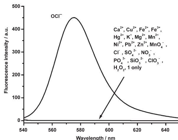
Figure 3. Fluorescence spectra ( \lambda_{\text{ex}}=520\text{ nm} ) of 1 ( 10\text{ }\mu\text{M} ) at pH 12 in the presence of 0.5–500 equivalents of various species (500 equiv of \text{Cl}^- or \text{K}^+ ; 100 equiv of \text{H}_2\text{O}_2 , \text{NO}_3^- , \text{PO}_4^{3-} , \text{SiO}_3^{2-} , or \text{SO}_4^{2-} ; 30 equiv of \text{Mg}^{2+} ; 15 equiv of \text{Ca}^{2+} ; 10 equiv of \text{ClO}_3^- , \text{Ni}^{2+} , or \text{Zn}^{2+} ; 2 equiv of \text{Mn}^{2+} ; 1 equiv of \text{Cu}^{2+} , \text{Fe}^{2+} , \text{MnO}_4^- , or \text{OCl}^- ; 0.5 equiv of \text{Fe}^{3+} , \text{Hg}^{2+} , or \text{Pb}^{2+} were used).
