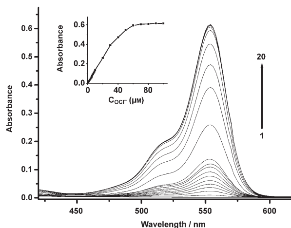
Figure 2. Absorption spectra of probe 1 (10 \mu\text{M} , curve 1) and its reaction solution with \text{OCl}^- at various concentrations (1–100 \mu\text{M} , curves 2–20) against the corresponding reagent blank. The reaction was carried out in 0.03 M \text{Na}_2\text{B}_4\text{O}_7/\text{NaOH} buffer (pH 12) that contained 30% (v/v) THF. The inset depicts the absorbance at the absorption maximum of 554 nm in the curves 2–20 as a function of \text{OCl}^- concentration.
