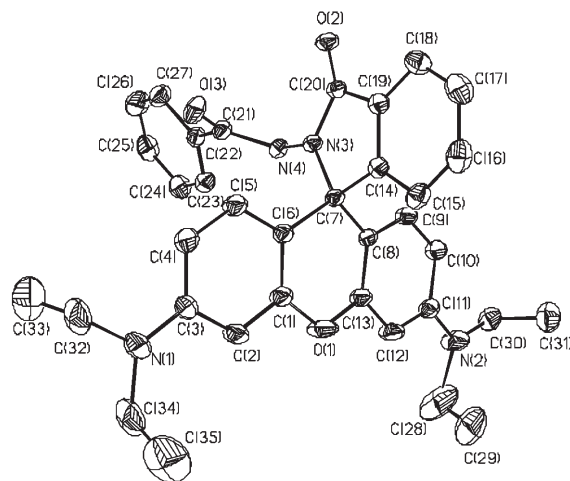
Figure 1. X-ray crystal structure of 1 .
